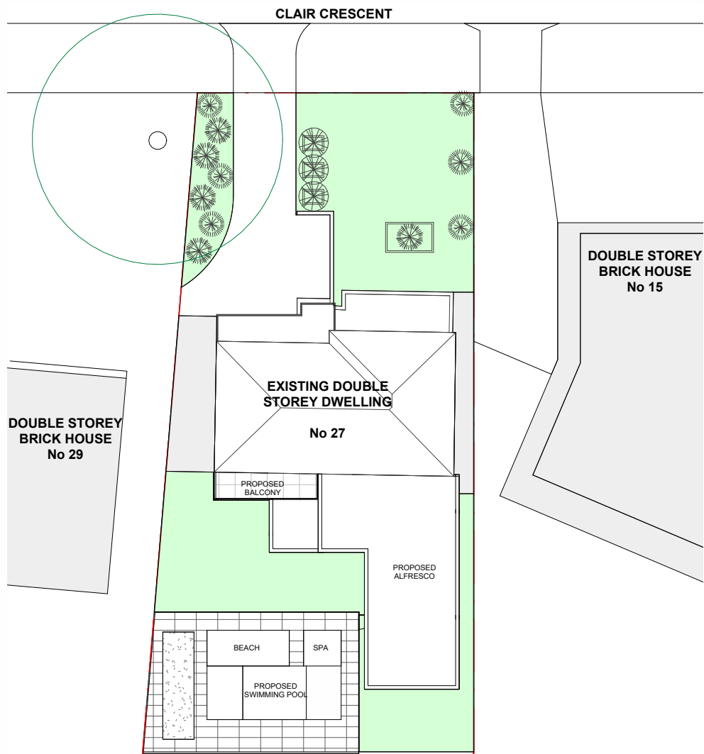
27 CLAIR CRESCENT - SITE PLAN
